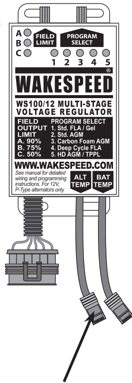
Alternator Temperature Sensor Cable
