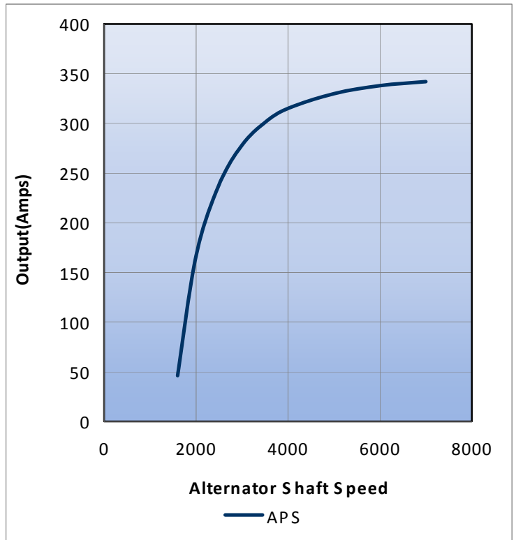
OUTPUT PERFORMANCE CURVE APS 360HPI Series Hot per SAE J56
